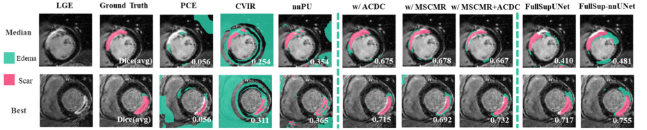
Fig. 3. The qualitative comparison on MyoPS dataset. The two images are the median and best cases selected by the average Dice Score.
